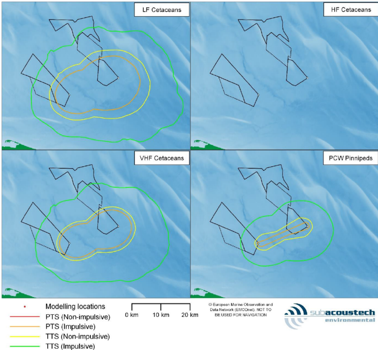
Figure 5-2 Contour plots showing the in-combination impacts of simultaneous installation of worst case monopile foundations at the SEP E and DEP SE modelling locations for marine mammals using the Southall et al. (2019) criteria assuming a fleeing receptor
