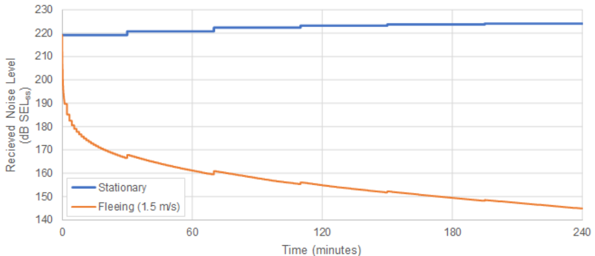
Figure 4-8 Received single-strike noise levels (SEL ss ) for receptors during the worst case monopile piling parameters assuming both a stationary and a fleeing receptor starting at a location 1 m from the noise source
